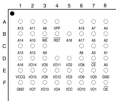
AT49BV1604(T) μBGA Top View (Ball Down)
