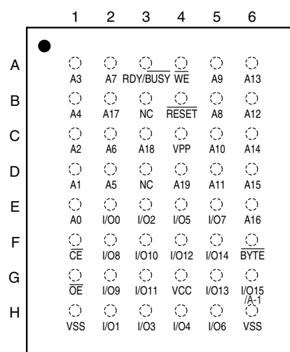
CBGA Top View
