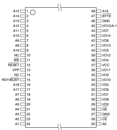
TSOP Top View Type 1
