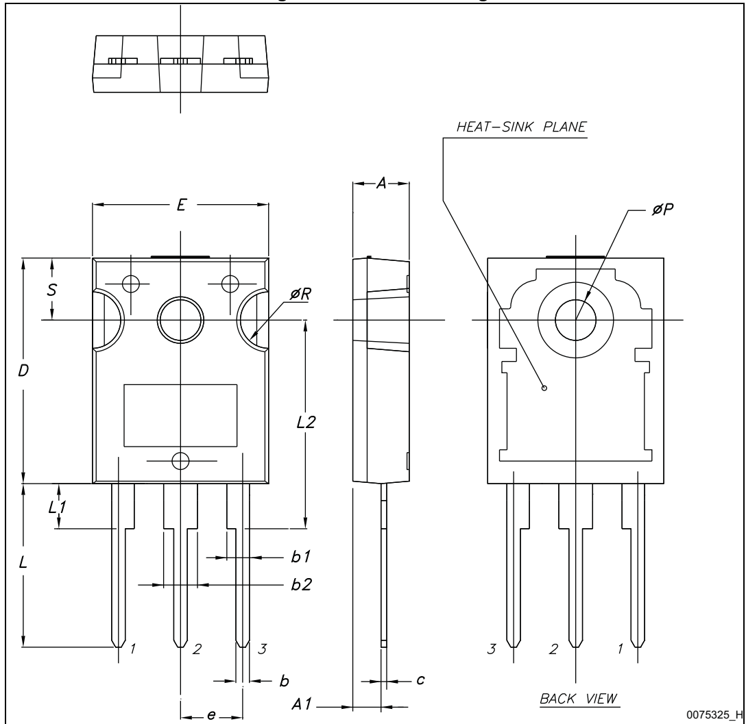
Figure 28. TO-247 drawing
