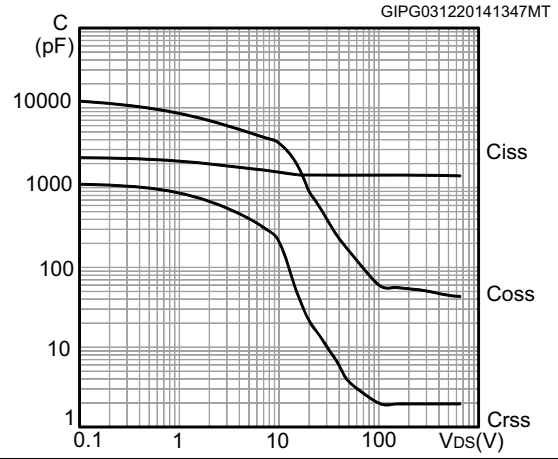
Figure 15. Capacitance variations
