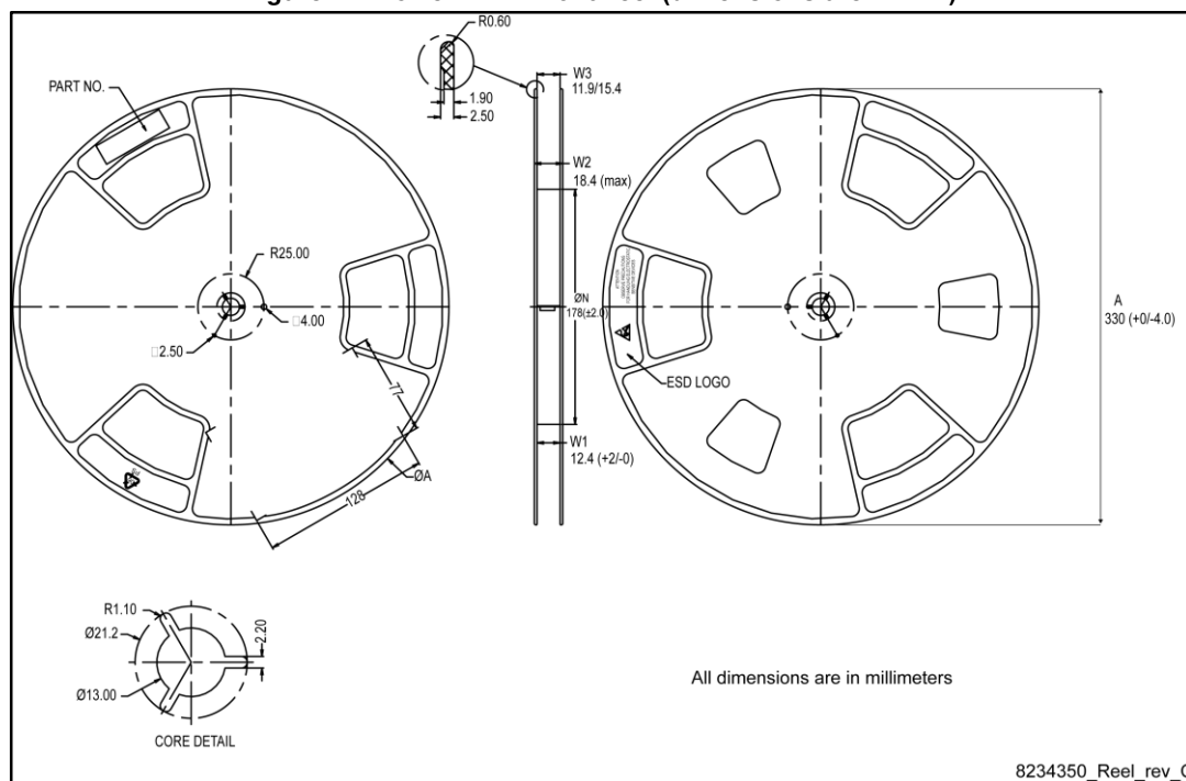
Figure 21: PowerFLAT™ 5x6 reel (dimensions are in mm)
