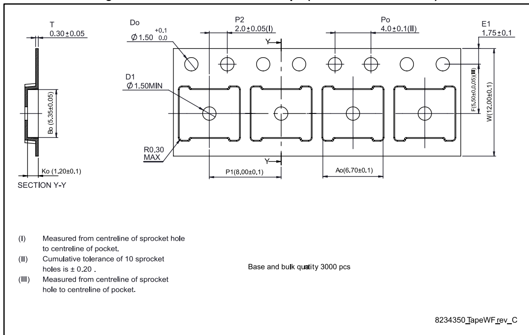
Figure 20: PowerFLAT™ 5x6 package orientation in carrier tape
