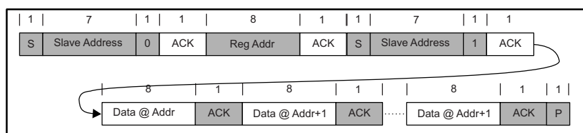
Figure 26. Multi-Read
