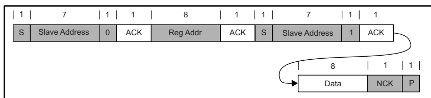
Figure 24. Single Read
