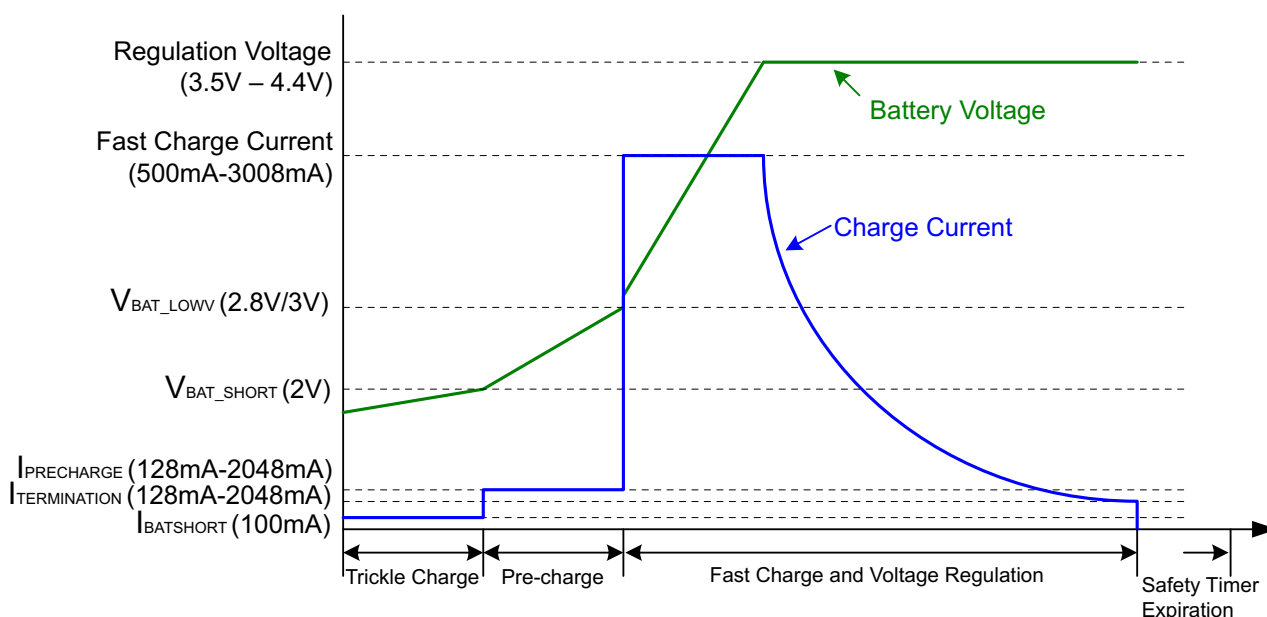
Figure 14. Battery Charging Profile
