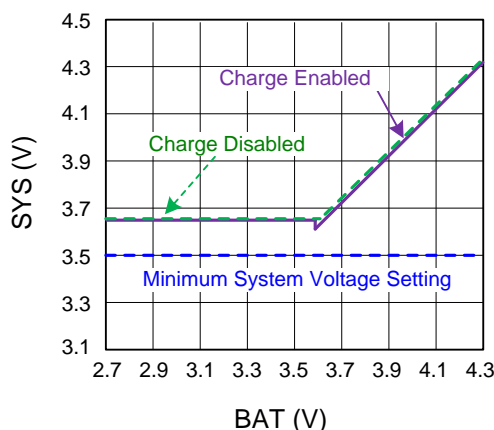
Figure 11. V(SYS) vs V(BAT)
