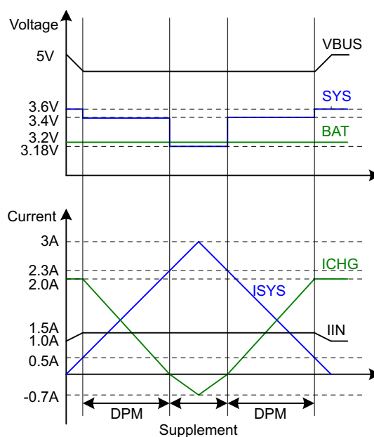
Figure 12. DPM Response
