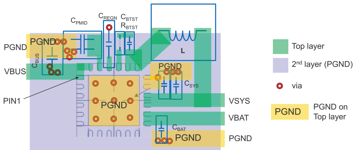
Figure 49. Layout Example
