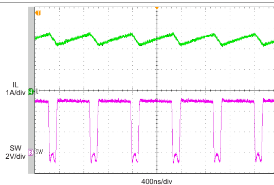
Figure 40. Charge Enable
