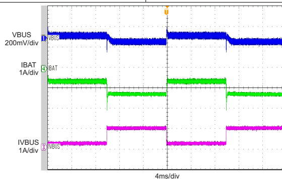
Figure 45. Load Transient During Supplement Mode
