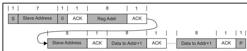
Figure 25. Multi-Write
