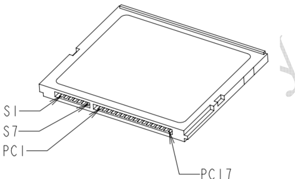
Figure 3-1 Pin Assignment
