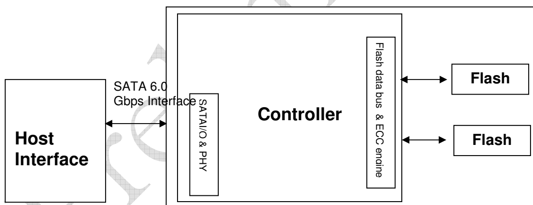
Figure 2-1 Apacer CFast STD block diagram
