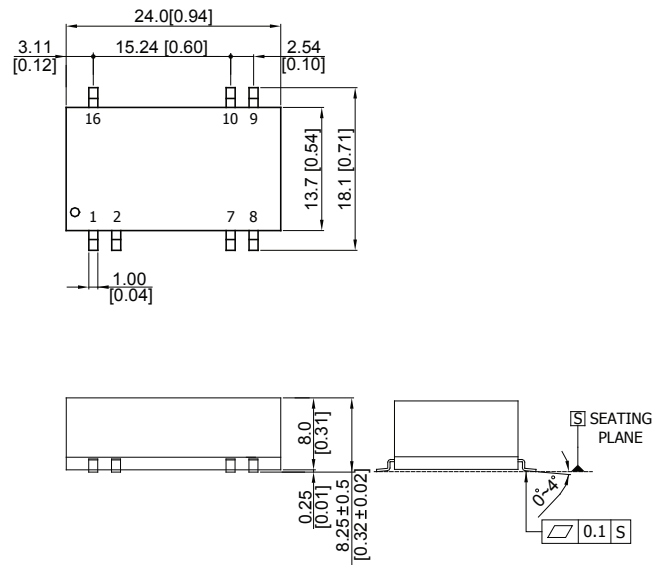
ATAxxxS-L (SMD)
