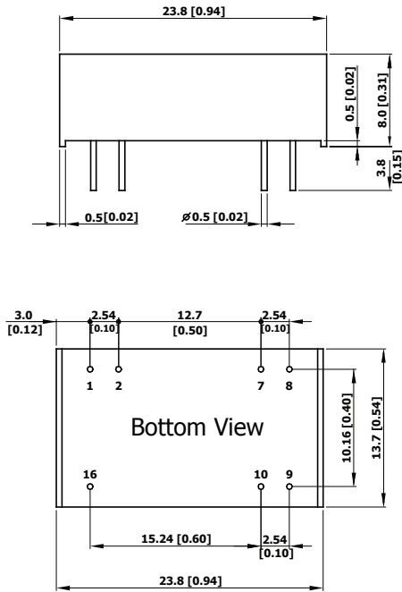
ATAxxx-L (DIP)
