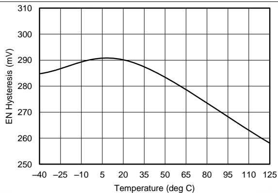
Figure 15. EN Hysteresis vs Junction Temperature
