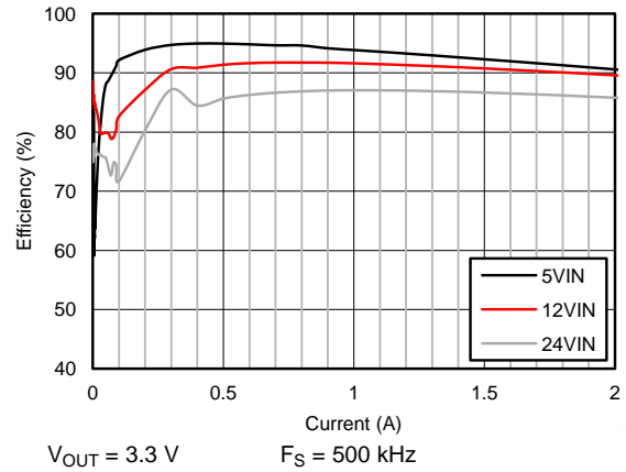
Figure 2. Efficiency at Room Temperature
