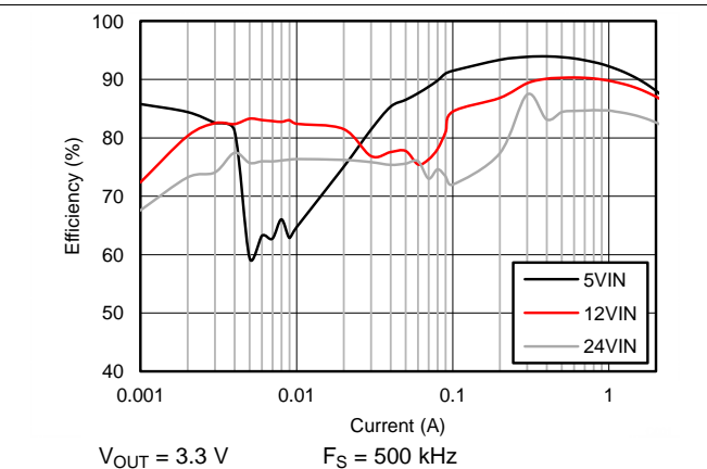
Figure 42. Efficiency at 85°C
