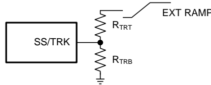
Figure 28. Soft Start Tracking External Ramp
