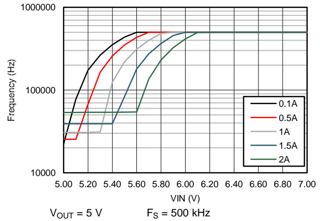
Figure 58. Frequency vs VIN
