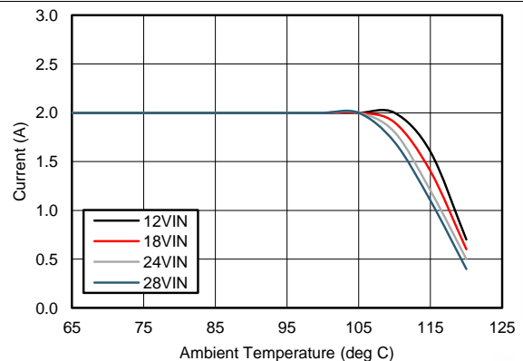
Figure 60. Regulation Curve
