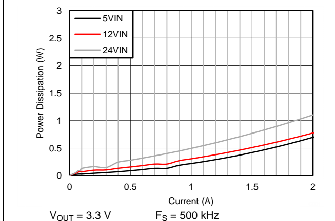
Figure 43. Power Loss at Room Temperature
