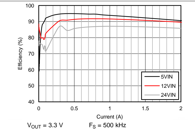
Figure 40. Efficiency at Room Temperature
