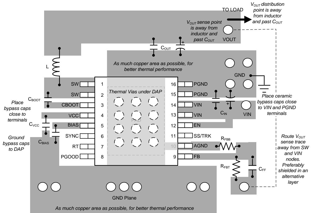
Figure 65. LM43602-Q1 Layout Example
