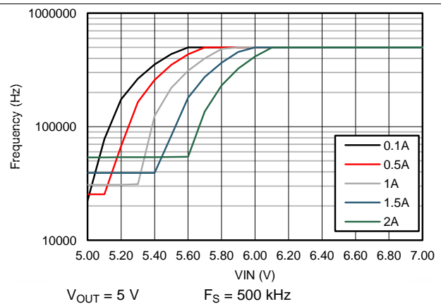
Figure 12. Frequency vs V_{IN}
