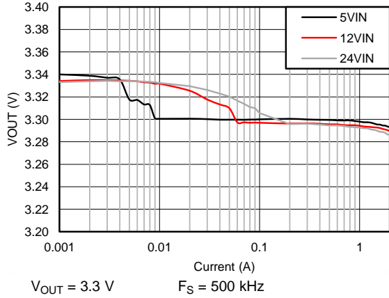
Figure 7. V_{OUT} Regulation
