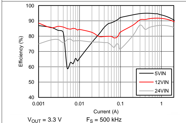
Figure 41. Efficiency at Room Temperature
