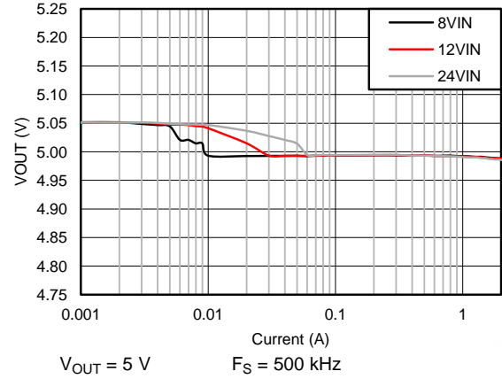
Figure 8. V_{OUT} Regulation
