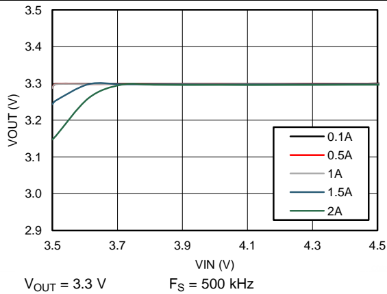
Figure 9. Dropout Curve
