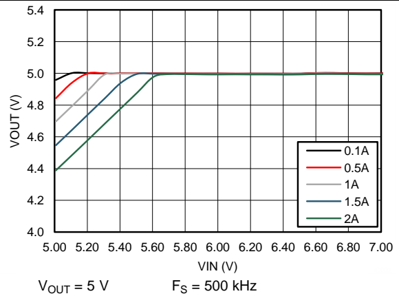
Figure 10. Dropout Curve
