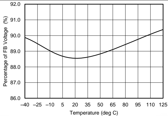
Figure 23. PGOOD UVP Falling Threshold vs Junction Temperature
