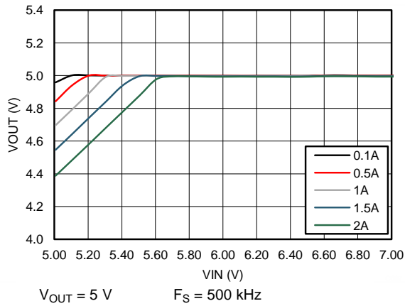
Figure 57. Dropout Voltage
