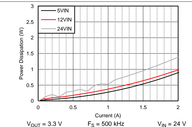
Figure 44. Power Loss at 85°C
