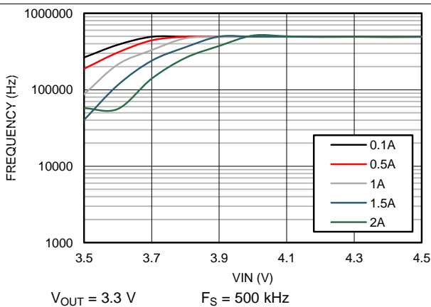
Figure 11. Frequency vs V_{IN}
