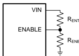
Figure 27. System UVLO by Enable Dividers
