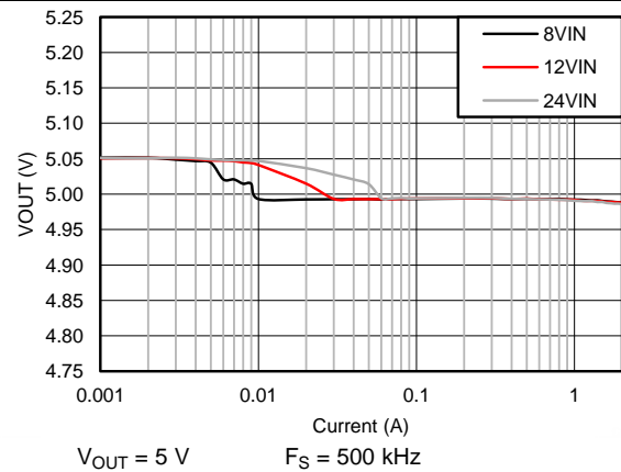
Figure 60. Regulation Curve
