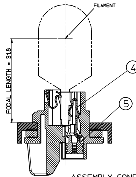
ASSEMBLY CONDITION
