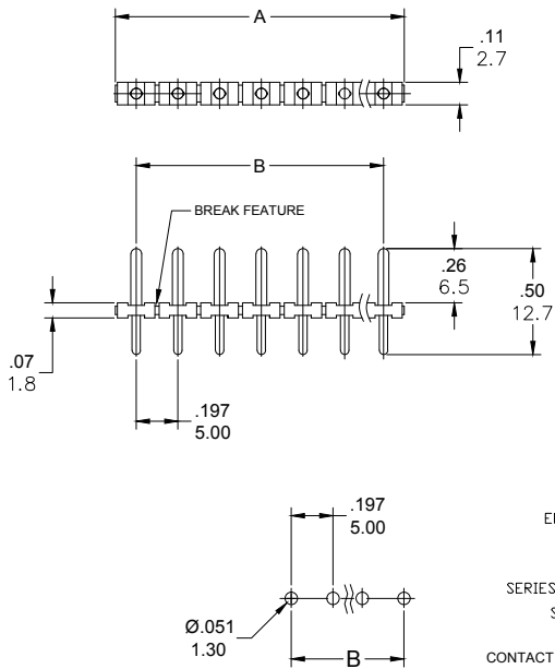
PCB LAYOUT
