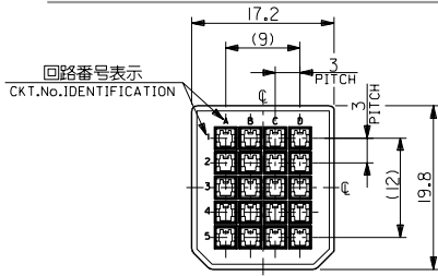
嵌合側 MATING SIDE
