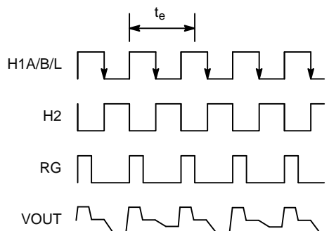
Figure 15. Pixel Timing
