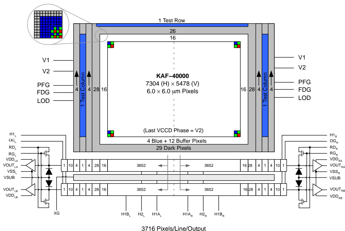
Figure 2. Block Diagram
