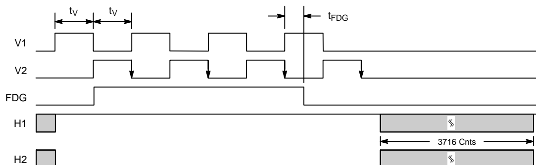
Figure 20. Line Dump Timing Example
