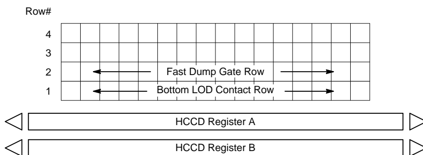
Figure 18. Fast Line Dump Layout
