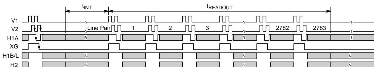
Figure 12. Frame Timing
