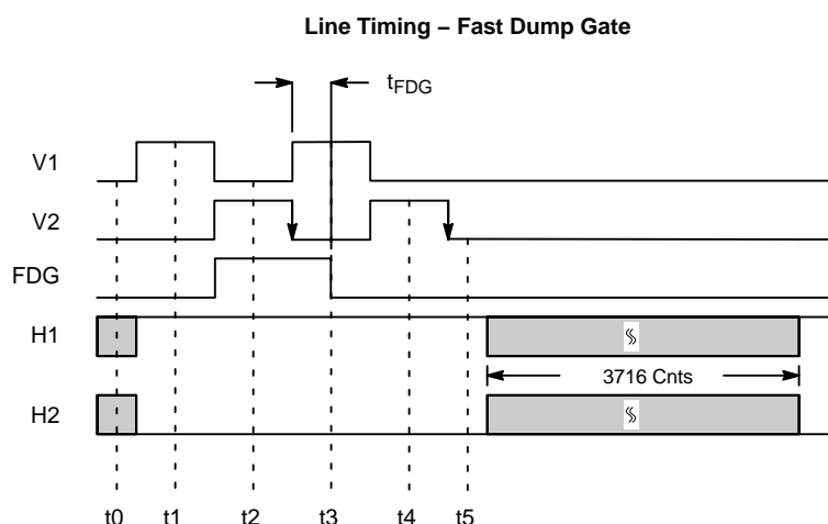
Figure 19. One Line Dump Timing Example
