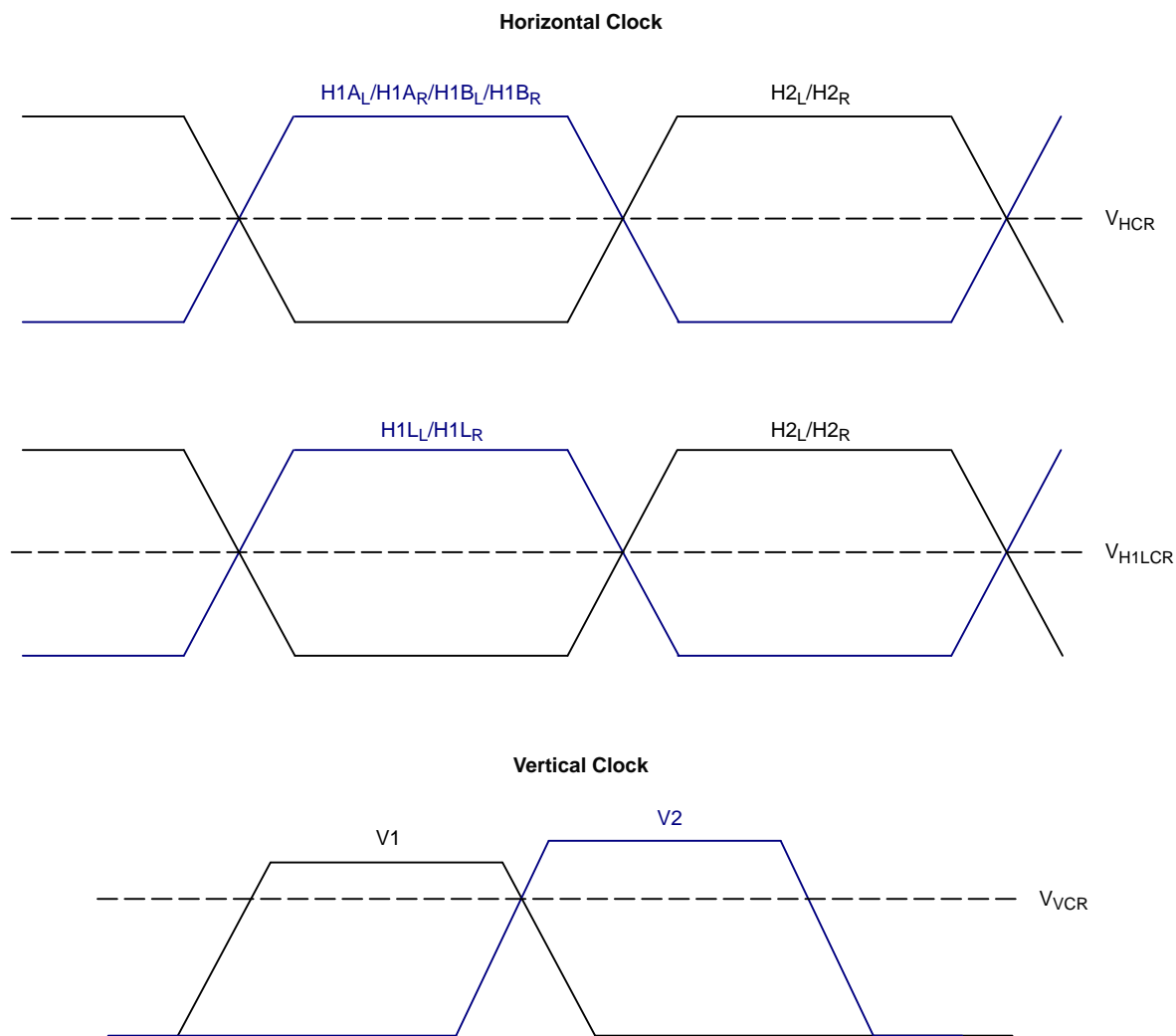
Figure 11. Timing Edge Alignment
