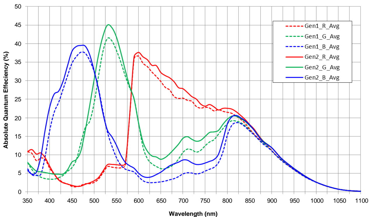
Figure 7. Spectral Response
