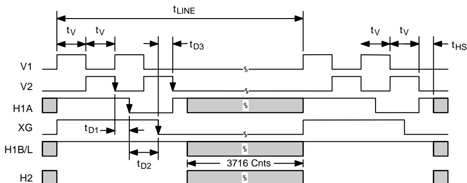
Figure 14. Line Timing
