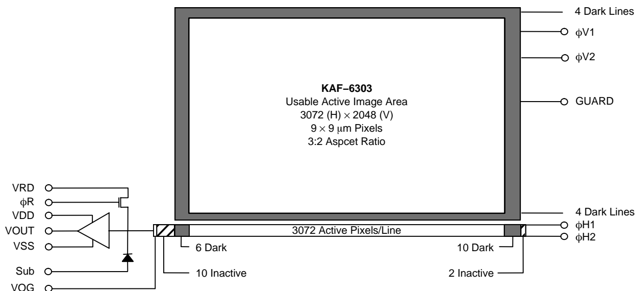
Figure 2. Block Diagram
