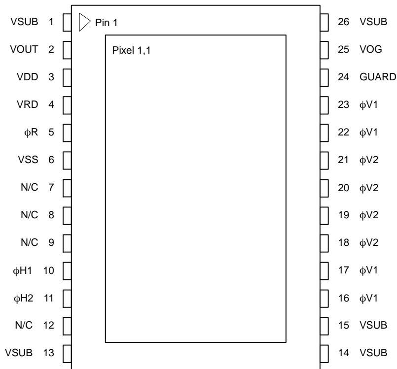
Figure 4. Pinout Diagram
