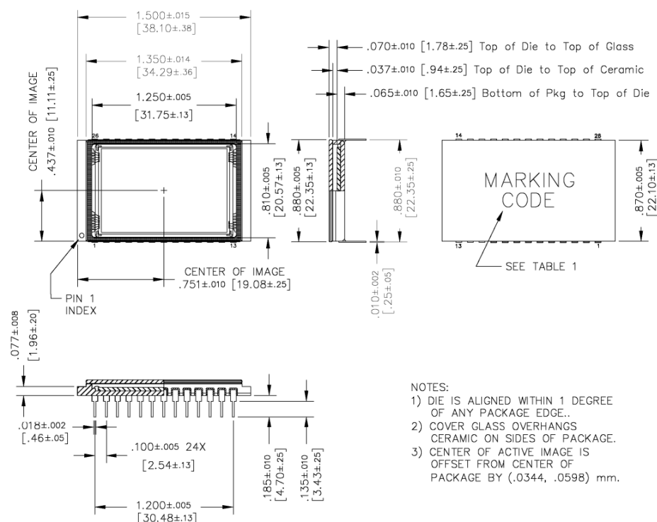
Figure 9. Completed Assembly (1 of 2)
