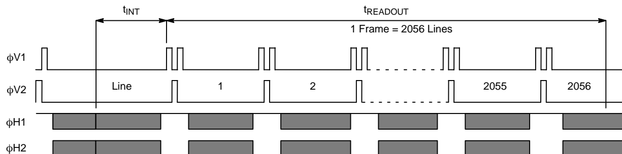
Figure 7. Frame Timing
