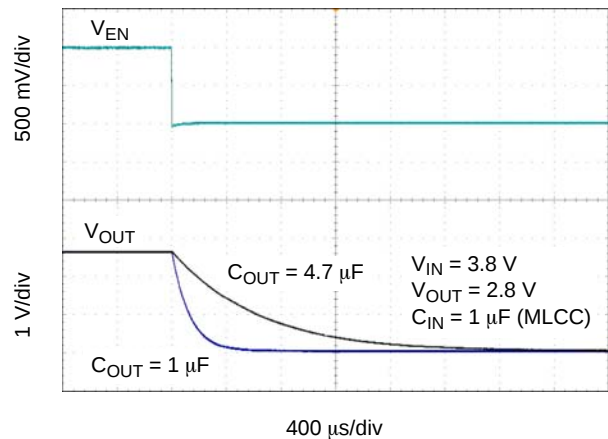
Figure 48. Enable Turn-off
