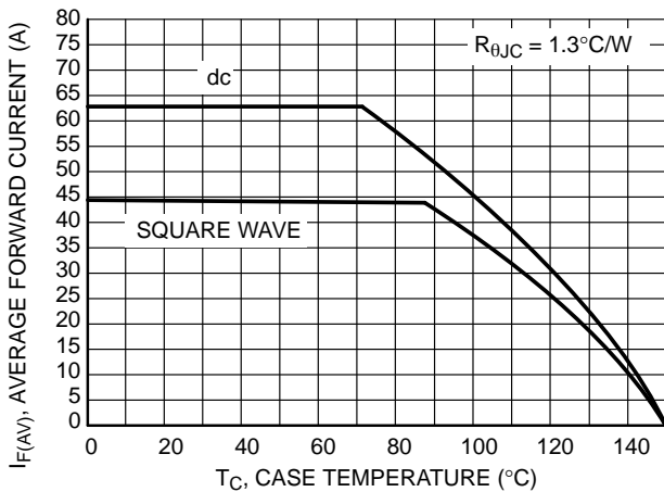
Figure 5. Current Derating, Case
