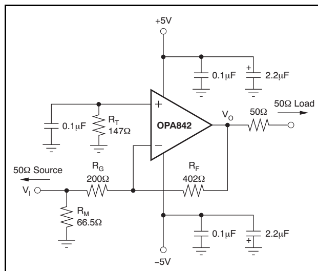
Figure 38. Inverting G = -2 Specifications and Test Circuit
