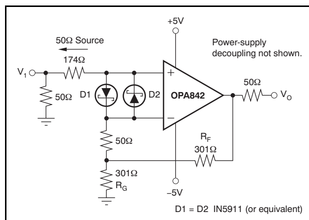
Figure 45. Gain of +2 with Input Protection
