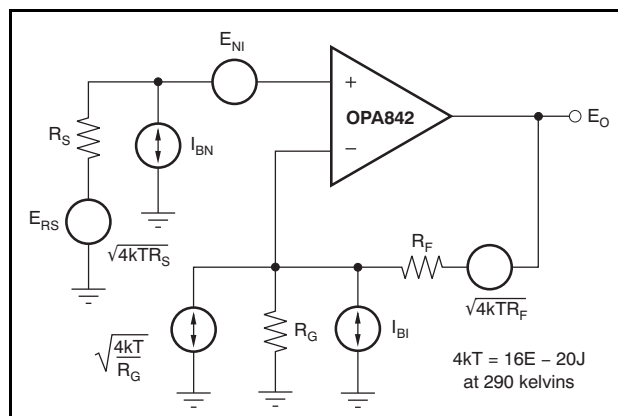
Figure 43. Op Amp Noise Analysis Model
