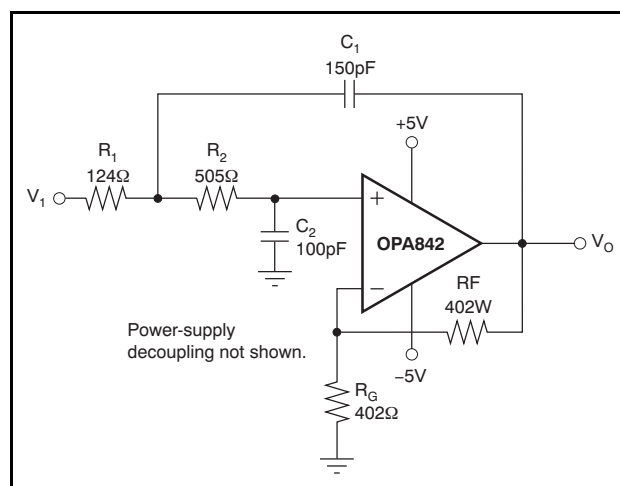
Figure 42. 5MHz Butterworth Low-Pass Active Filter
