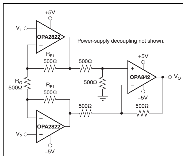
Figure 40. Wideband Three-Op Amp Differencing Amplifier
