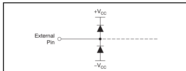
Figure 44. Internal ESD Protection
