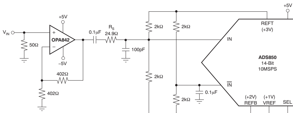
AC-Coupled to 14-Bit ADS850 Interface
