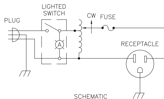
SCHEMATIC
