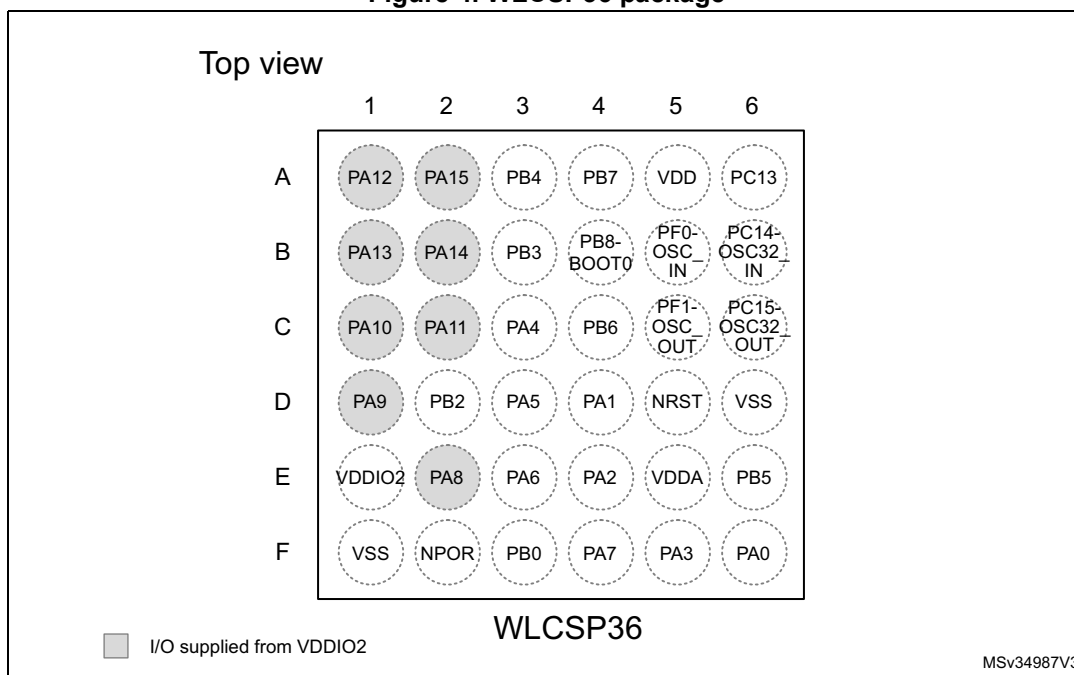
Figure 4. WLCSP36 package
