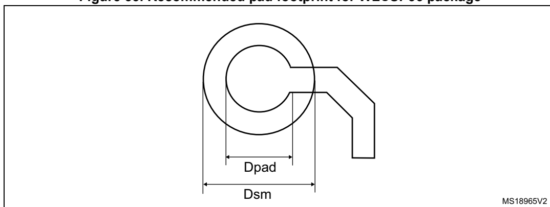
Figure 33. Recommended pad footprint for WLCSP36 package
