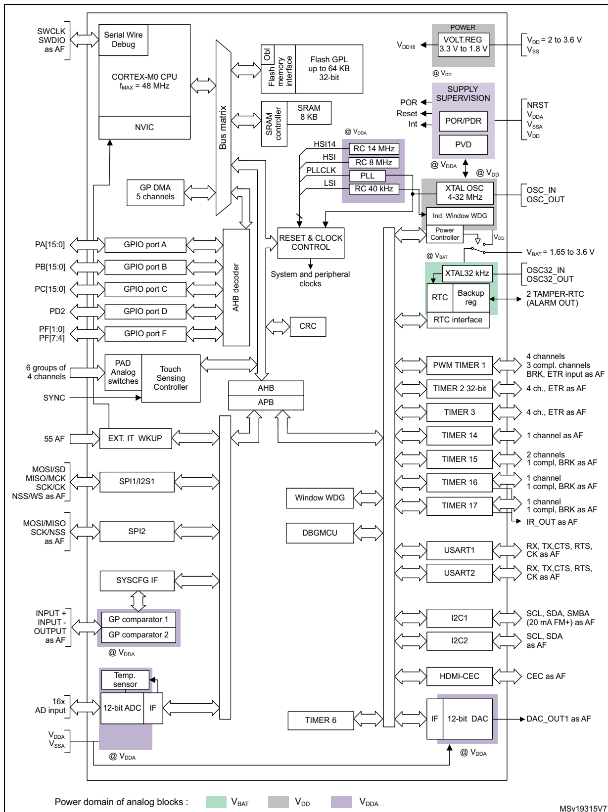
Figure 1. Block diagram
