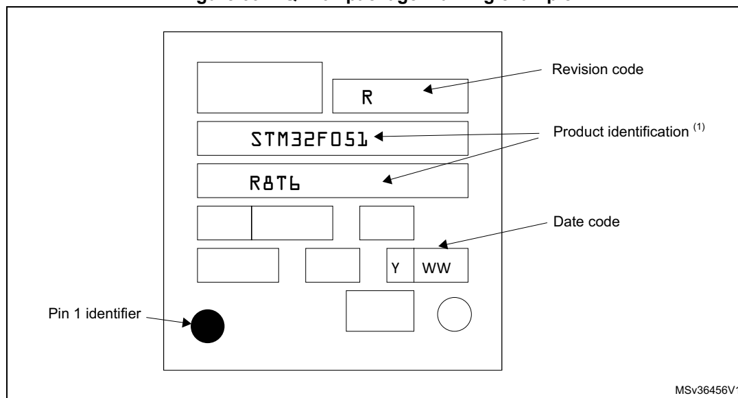
Figure 39. LQFP64 package marking example
