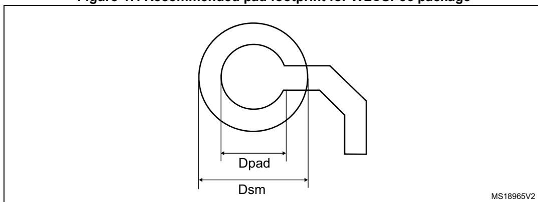
Figure 47. Recommended pad footprint for WLCSP36 package
