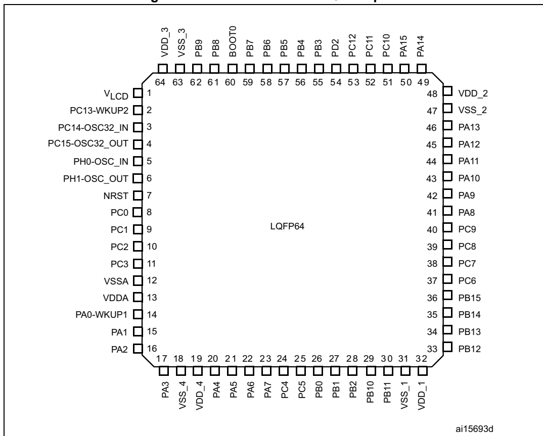
Figure 6. STM32L15xRxxxA LQFP64 pinout
