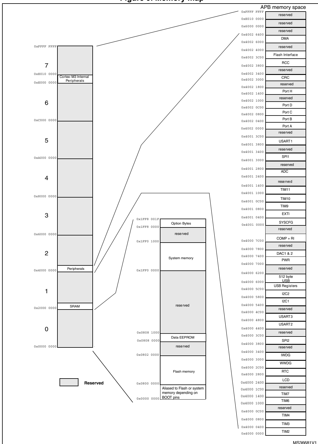
Figure 9. Memory map
