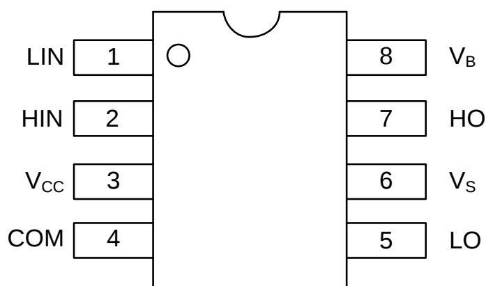
8-Lead SOIC
