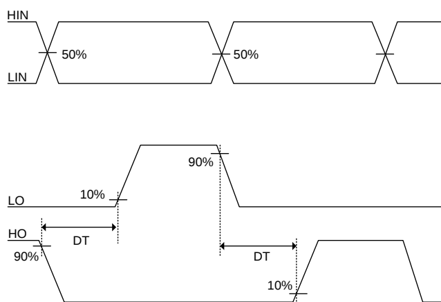
Figure X. Internal Deadtime Timing
