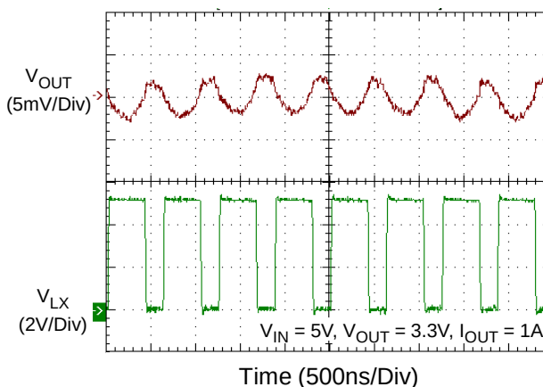
Voltage Ripple
