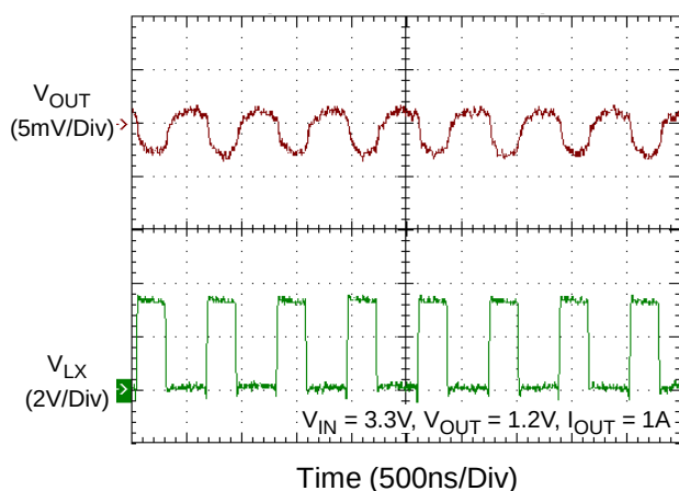
Voltage Ripple
