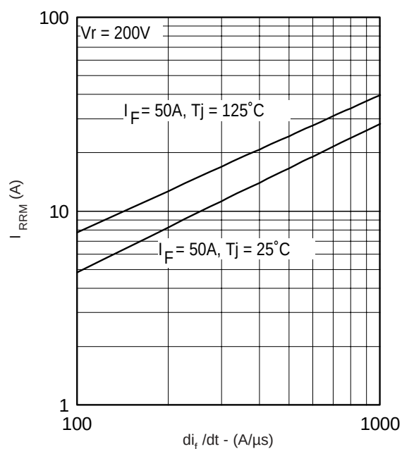
Fig. 7 - Typical Reverse Recovery Current vs. di/dt
