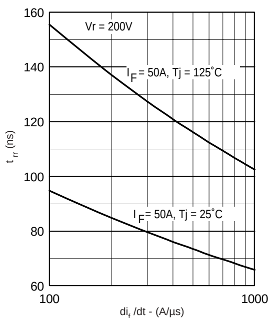
Fig. 6 - Typical Reverse Recovery vs. di/dt
