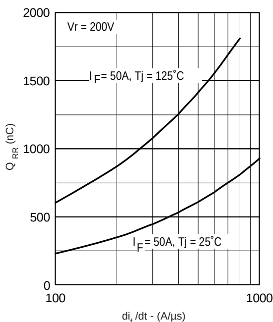
Fig. 8 - Typical Stored Charge vs. di/dt
