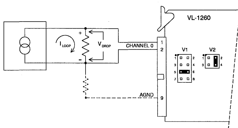
Figure 2-12. Current Loop Input Mode
