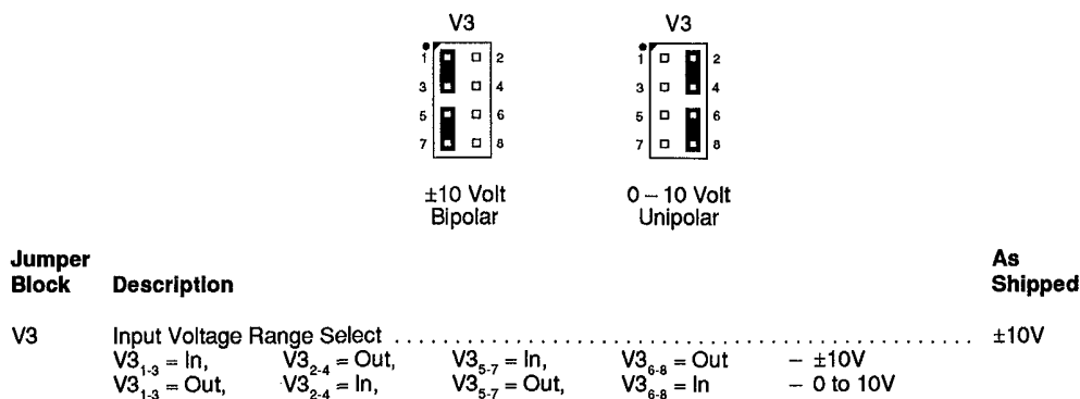
Figure 2-13. Input Range Selection
