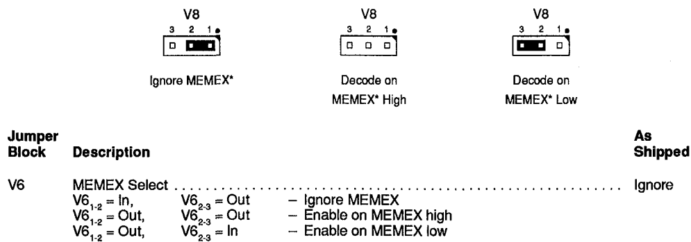
Figure 2-8. MEMEX Options
