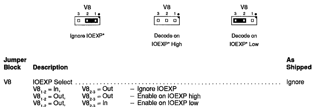
Figure 2-6. IOEXP Options
