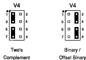
Figure 2-15. Valid Input Data Formats
