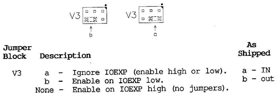
Figure 2-5. IOEXP Options
