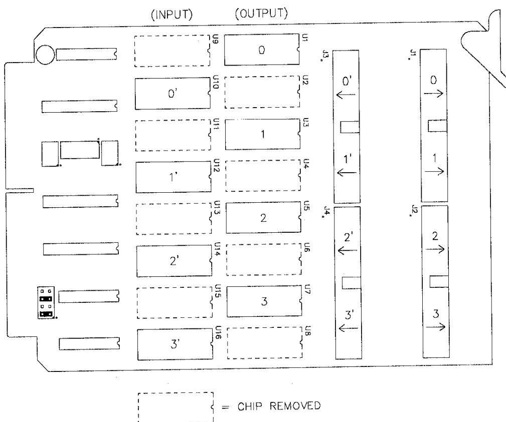
Figure 2-9. Special 4-Port Mode Configuration
