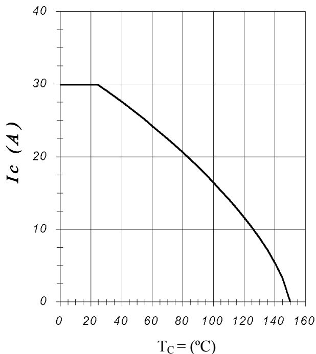
Fig. 1 – Maximum DC collector Current vs. case temperature
