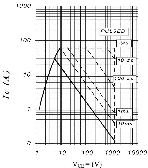
Fig. 3 – Forward SOA T_c = 25^{\circ}\text{C} ; T_j \leq 150^{\circ}\text{C}
