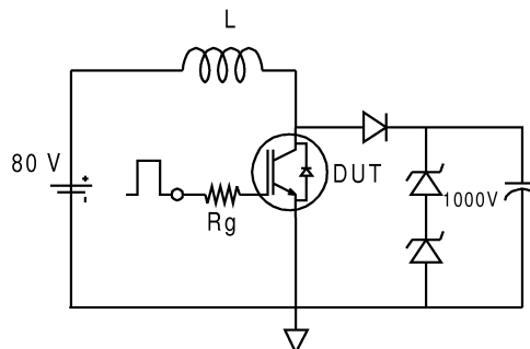
Fig. CT.2 - RBSOA Circuit
