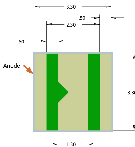
Bottom View
