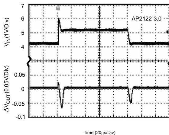
Figure 17. Line Transient (Conditions: I_{OUT}=30mA , C_{IN}=1\mu F , C_{OUT}=1\mu F )
