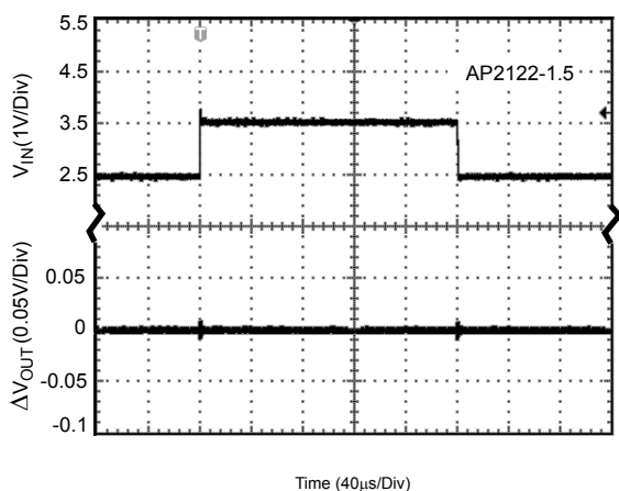
Figure 16. Line Transient (Conditions: I_{OUT}=30mA , C_{IN}=1\mu F , C_{OUT}=1\mu F )
