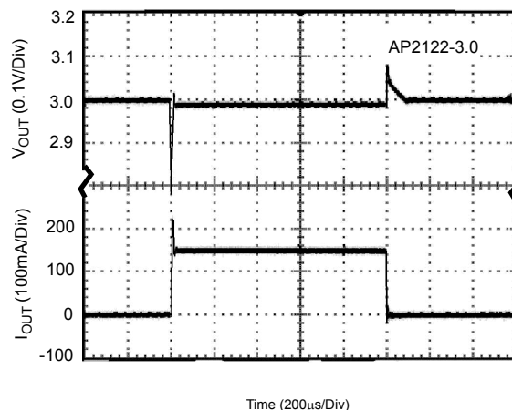
Figure 19. Load Transient (Conditions: V_{IN}=4V , C_{IN}=1\mu F , C_{OUT}=1\mu F )
