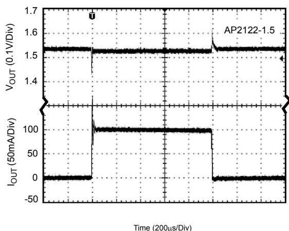
Figure 18. Load Transient (Conditions: V_{IN}=2.5V , C_{IN}=1\mu F , C_{OUT}=1\mu F )
