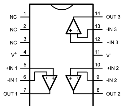
Figure 2. SOIC-14/TSSOP-14 (LMH6683) Top View
