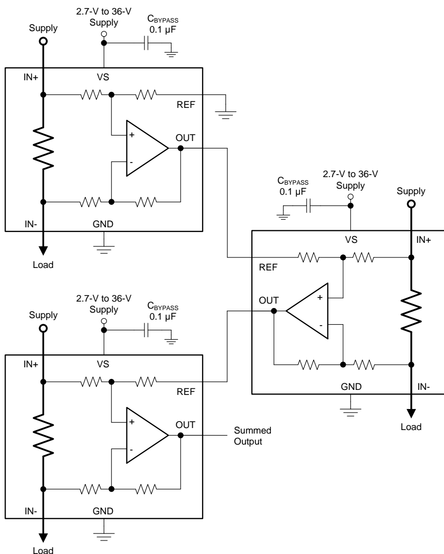
Figure 37. Daisy-Chain Configuration
