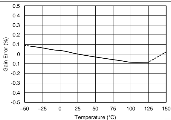
Figure 13. System Gain Error vs Temperature
