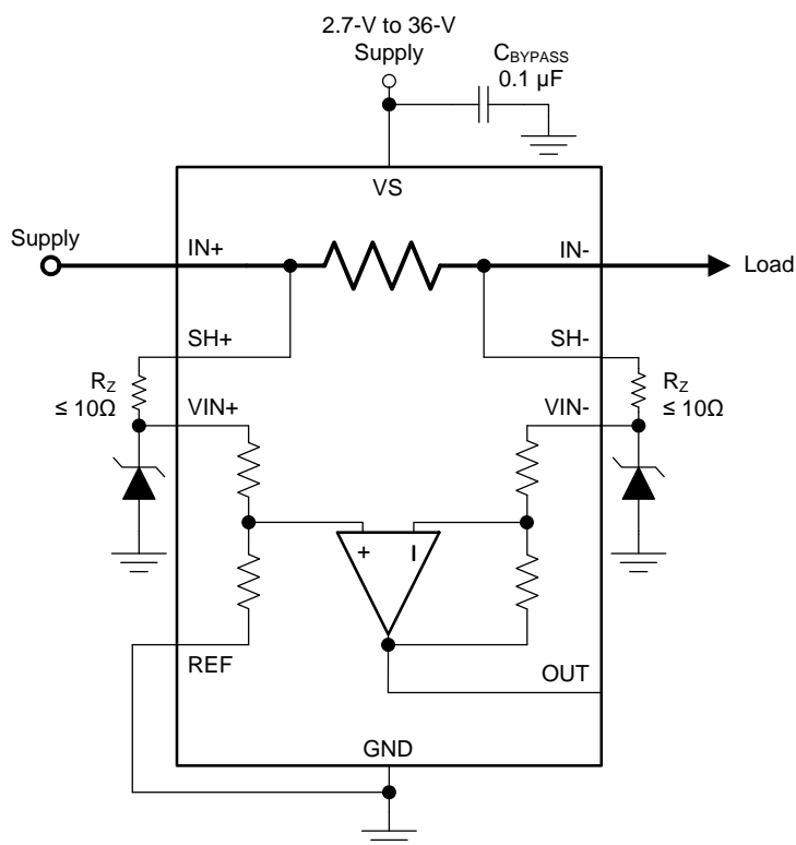
Figure 36. Device Transient Protection
