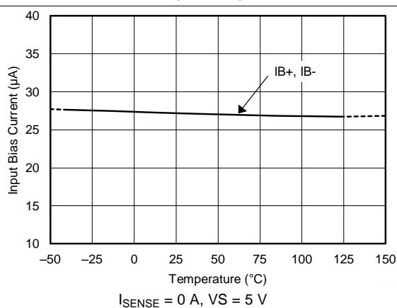
Figure 22. Input Bias Current vs Temperature
