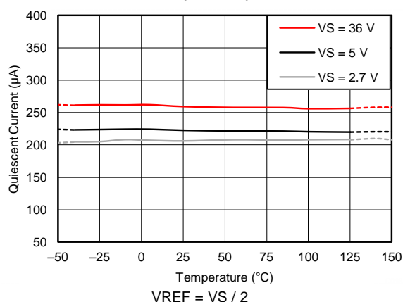
Figure 23. Quiescent Current vs Temperature
