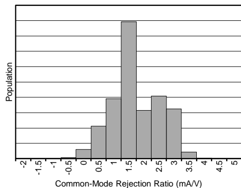
Figure 7. INA250A2 Common-Mode Rejection Ratio Distribution
