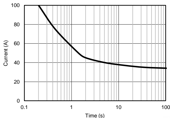
Figure 31. Short-Circuit Duration
