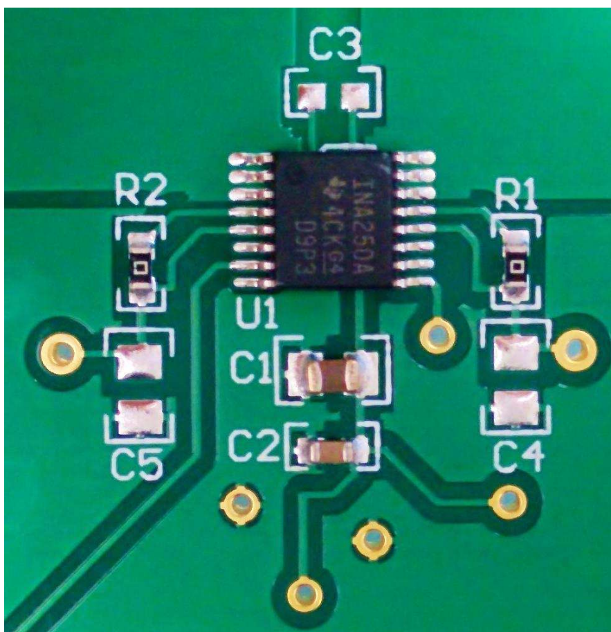
Figure 43. Recommended Layout
