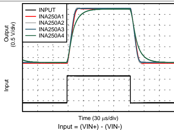
Figure 27. Step Response
