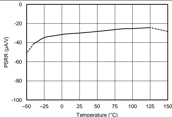
Figure 12. Power-Supply Rejection Ratio vs Temperature
