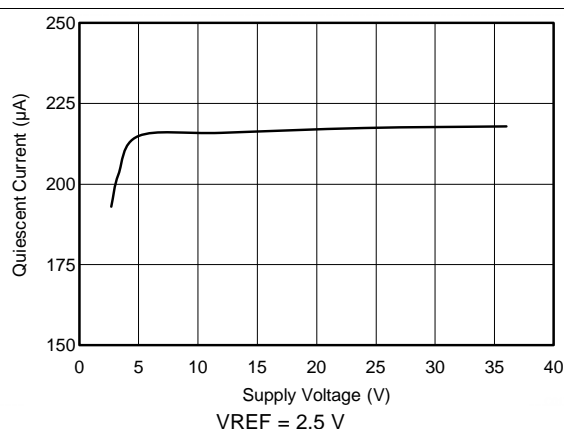
Figure 24. Quiescent Current vs Supply Voltage
