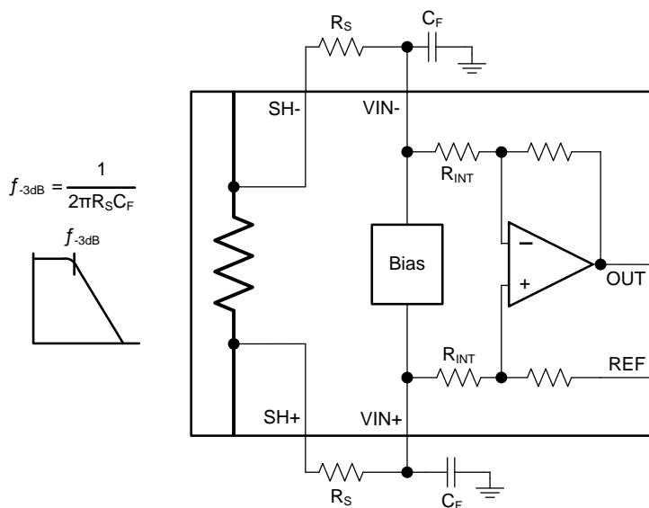
Figure 33. Input Filter
