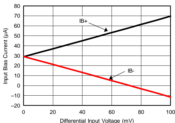
Figure 34. Input Bias Current vs Differential Input Voltage
