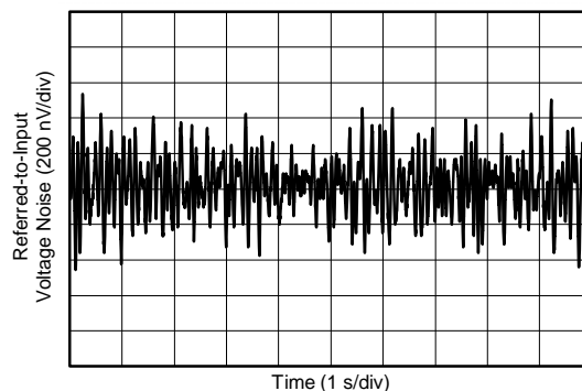
Figure 26. 0.1-Hz to 10-Hz Voltage Noise (Referred-to-Input)
