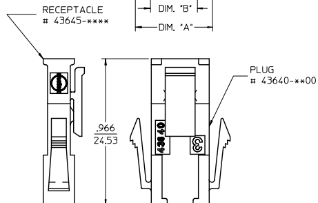
MATED MICRO-FIT CONNECTOR
