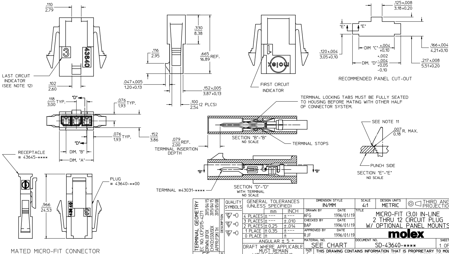
PLUG WITH PANEL MOUNTS
