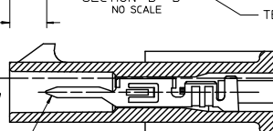
SECTION "D"- "D" WITH TERMINAL NO SCALE
