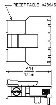
MATED MICRO FIT CONNECTOR
