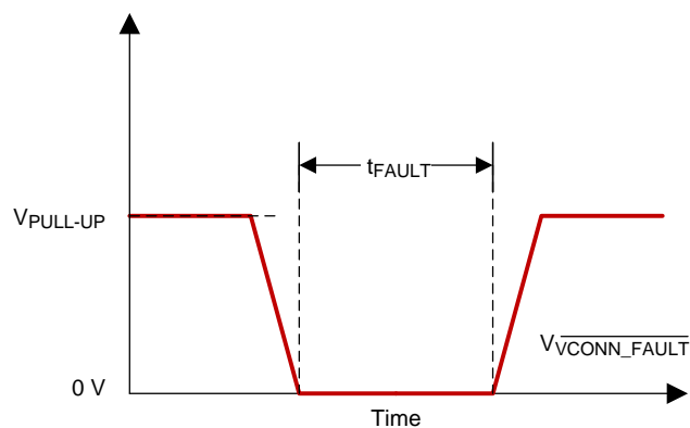
Figure 2. VCONN_FAULT Assertion Pulse Timing
