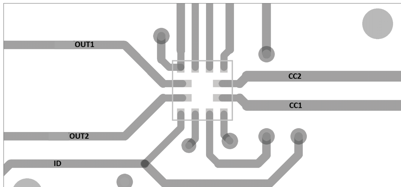
Figure 6. TUSB321 Layout
