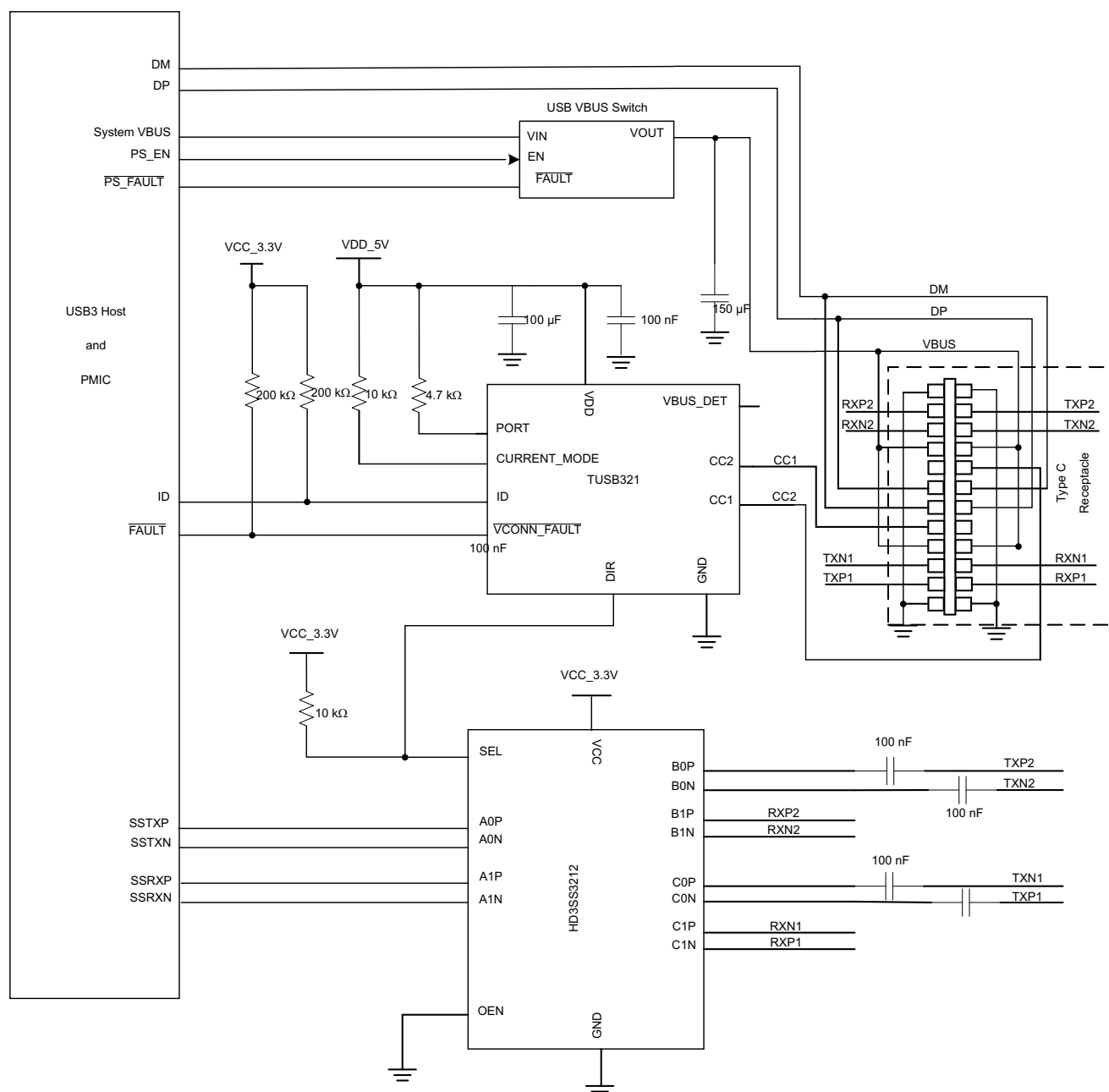
Figure 4. DFP Mode Schematic
