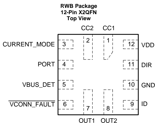
Pin Functions
