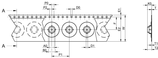
sectional drawing A-A
