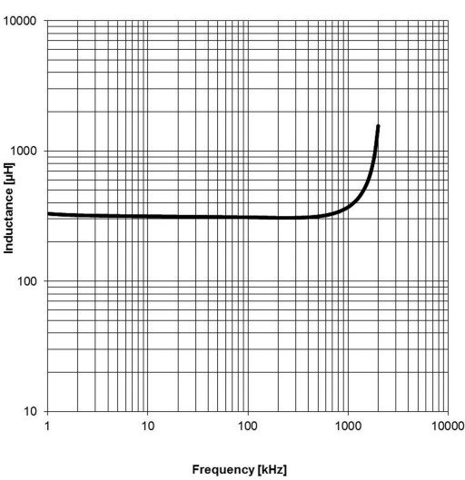
F2 Typical Inductance vs. Frequency Characteristics:
