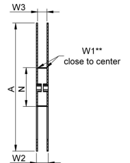
sectional drawing B-B
