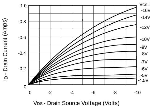
Saturation Characteristics
