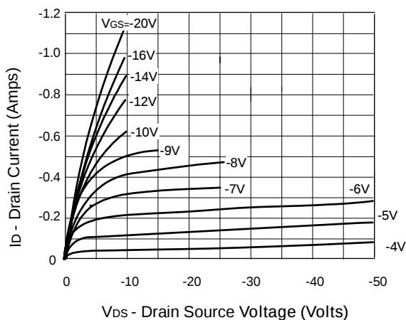
Output Characteristics
