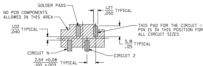
4 CIRCUIT SHOWN
