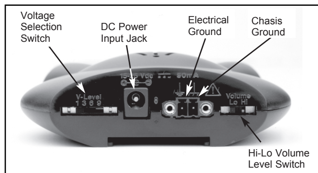
Figure 9. Rear of SCS Static Monitor 790.
