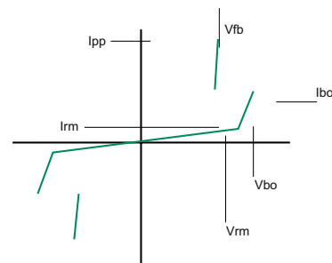
V-I Characteristic
