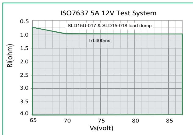
Figure 7 - SOA Chart
