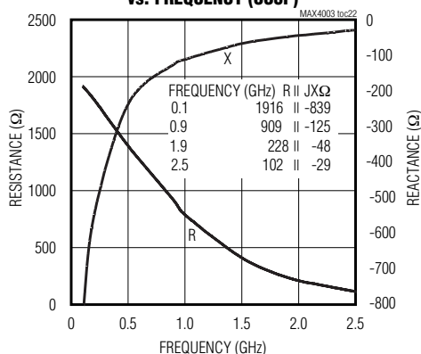
RFIN INPUT IMPEDANCE vs. FREQUENCY (UCSP)
