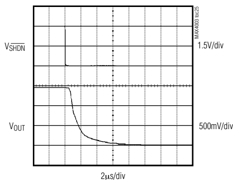
POWER-DOWN RESPONSE TIME
