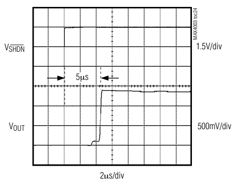
POWER-ON RESPONSE TIME
