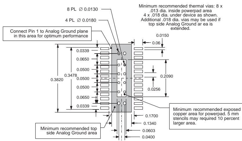
Figure 9. Recommended Land Pattern for 28-Pin PWP PowerPAD
