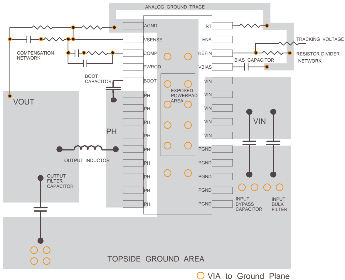
Figure 8. TPS54872 PCB Layout
