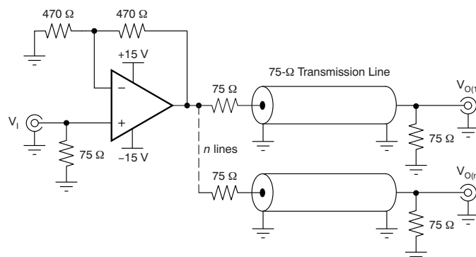
Figure 40. Video Distribution Amplifier Application
