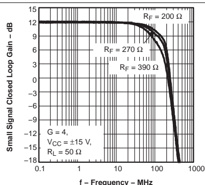
Figure 8. Small-Signal Closed-Loop Gain vs Frequency
