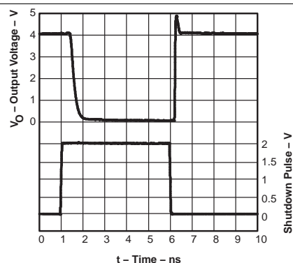
Figure 32. THS3125 Shutdown Response
