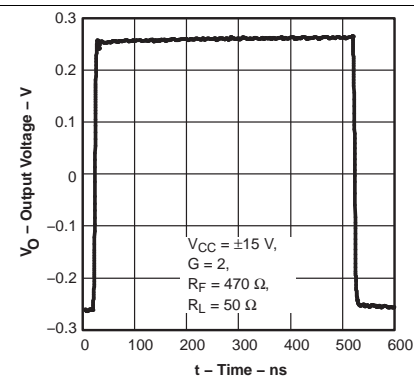
Figure 34. Small-Signal Pulse Response
