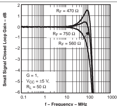
Figure 1. Small-Signal Closed-Loop Gain vs Frequency
