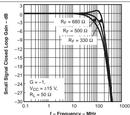
Figure 2. Small-Signal Closed-Loop Gain vs Frequency
