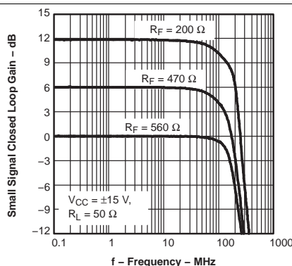
Figure 8. Small-Signal Closed-Loop Gain vs Frequency
