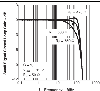
Figure 2. Small-Signal Closed-Loop Gain vs Frequency
