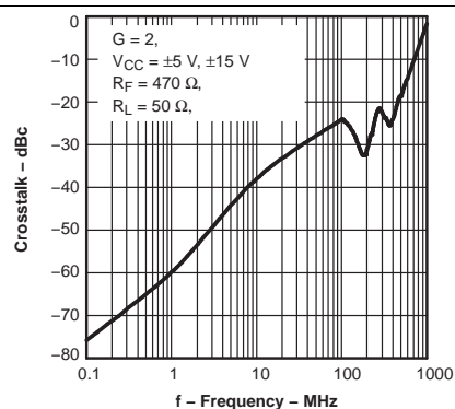
Figure 20. Crosstalk vs Frequency
