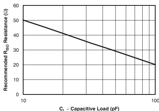
Figure 41. Recommended R ISO vs Capacitive Load
