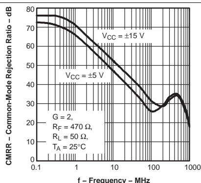
Figure 19. Common-Mode Rejection Ratio vs Frequency
