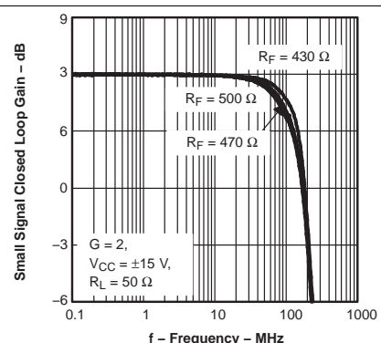
Figure 4. Small-Signal Closed-Loop Gain vs Frequency
