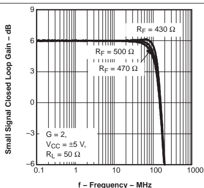
Figure 3. Small-Signal Closed-Loop Gain vs Frequency
