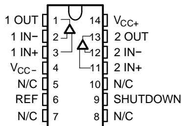
THS3125: D and PWP Packages SOIC-14 and HTSSOP-14 Top View
