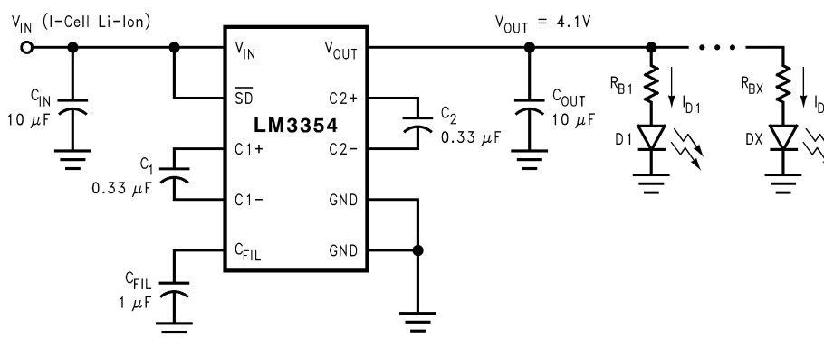
Figure 13. White LED Driver
