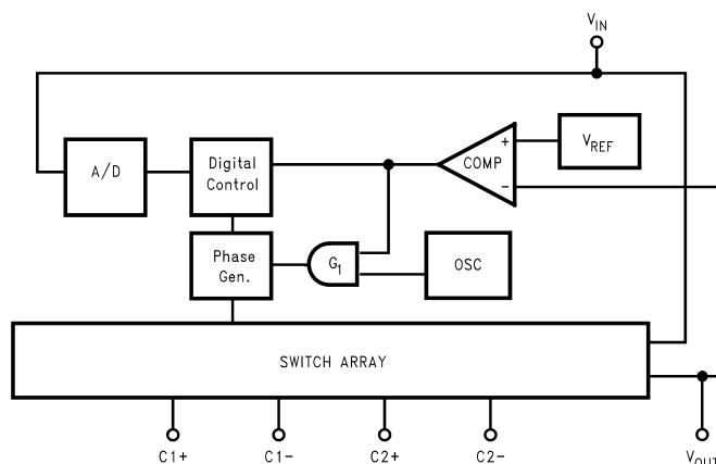
Figure 10. Block Diagram
