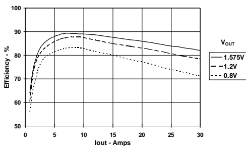
Efficiency vs Output Current
