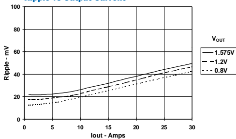
Ripple vs Output Current
