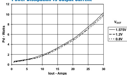
Power Dissipation vs Output Current
