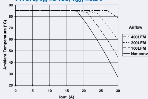
PT7673, V_{in} = 5 VDC , V_{out} = 1.2 V
