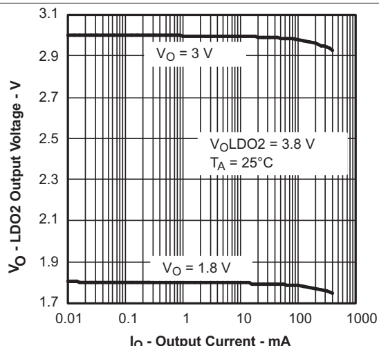
Figure 10. LDO2 Output Voltage vs Output Current
