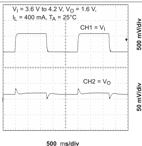
Figure 12. Line Transient Response (CORE)
