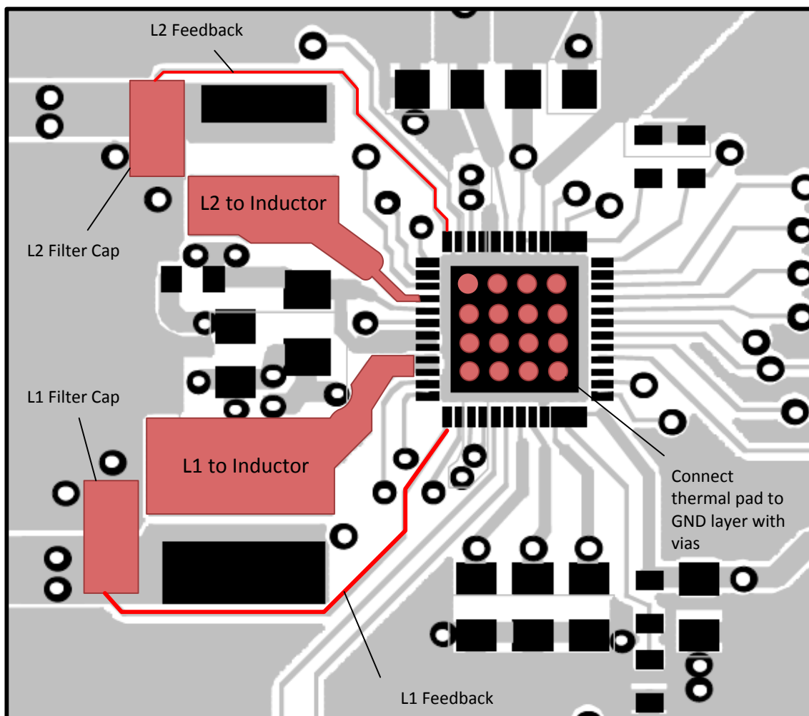
Figure 46. EVM Layout
