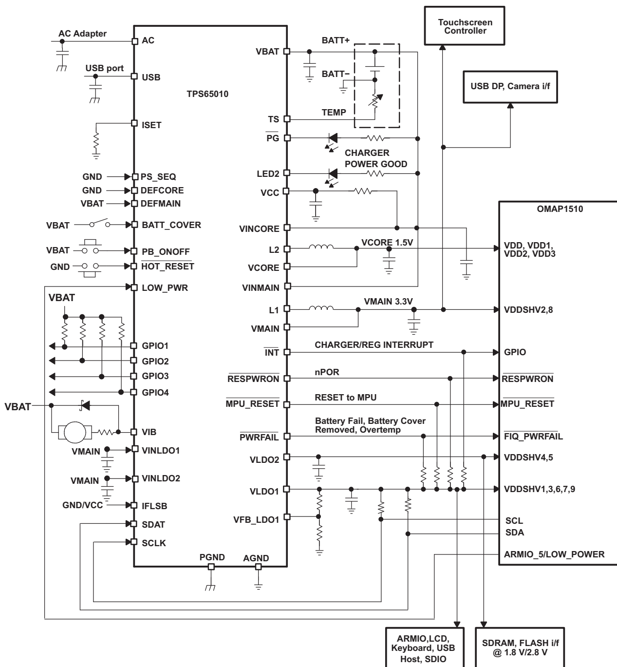
Figure 45. Typical Application Circuit in Low-Power Mode
