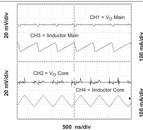
Figure 20. Output Ripple (PWM)
