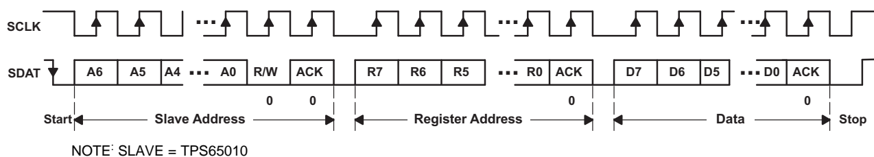
Figure 38. Serial Interface WRITE to TPS65010 Device
