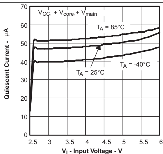
Figure 5. Quiescent Current vs Input Voltage
