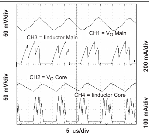
Figure 19. Output Ripple (PFM)
