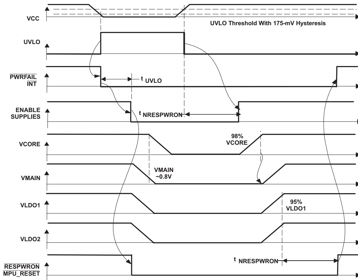
Figure 32. State2-State4-State 2 Transition
