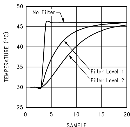
Figure 12. Step Response
