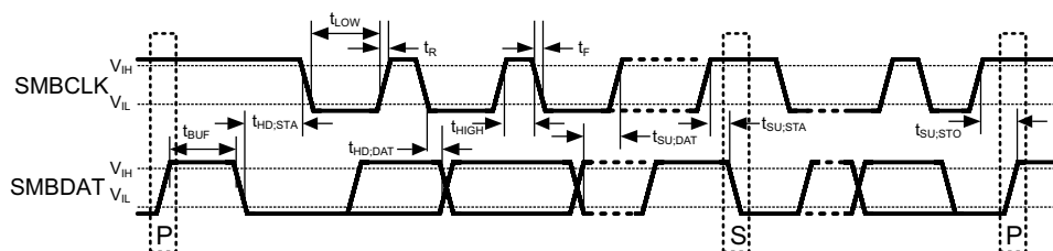
Figure 2. SMBus Communication
