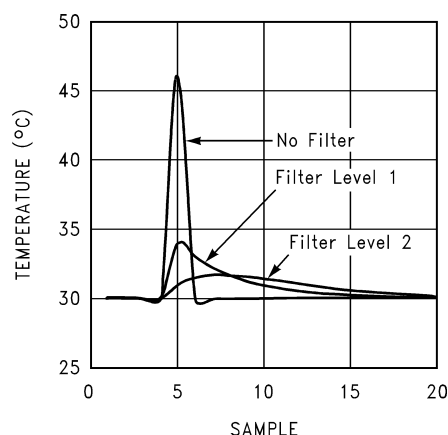
Figure 13. Impulse Response
